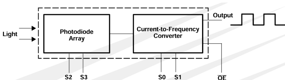
Figure 3-13: Block Diagram of TCS3200
