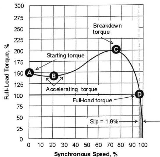
Figure 0-1: Typical Speed/Torque Curve for a NEMA-B Induction Motor
