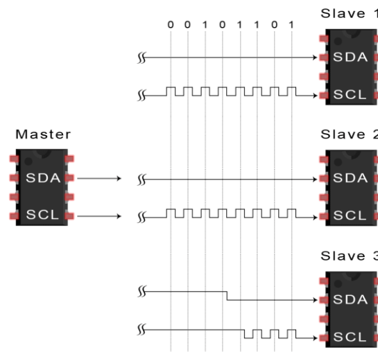
Figure 0-3: I2C Block Diagram
