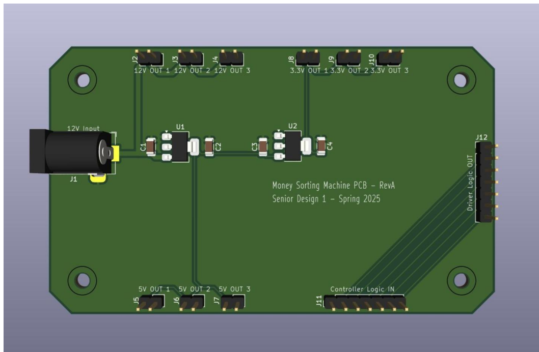
Figure 8-2: PCB 3D Front View
