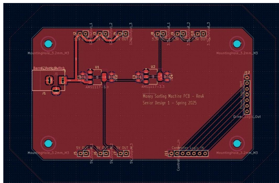
Figure 8-1: PCB 2D View
