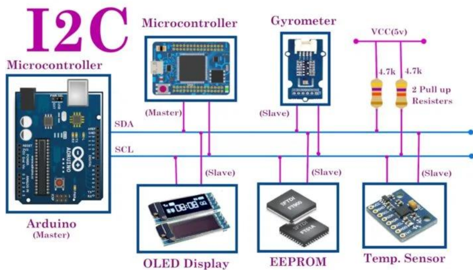
Figure 0-4: Example Diagram of I2C Communication
