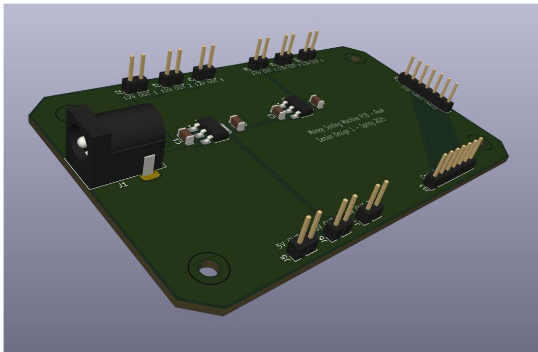
Figure 8-3: PCB 3D Angled View
