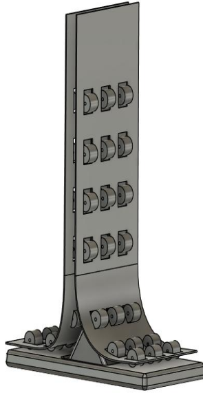
Figure 6-3: Flipper Mechanism
