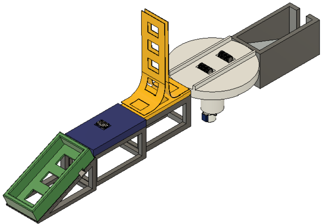
Figure 8-4: Complete Bill Orientation Design
