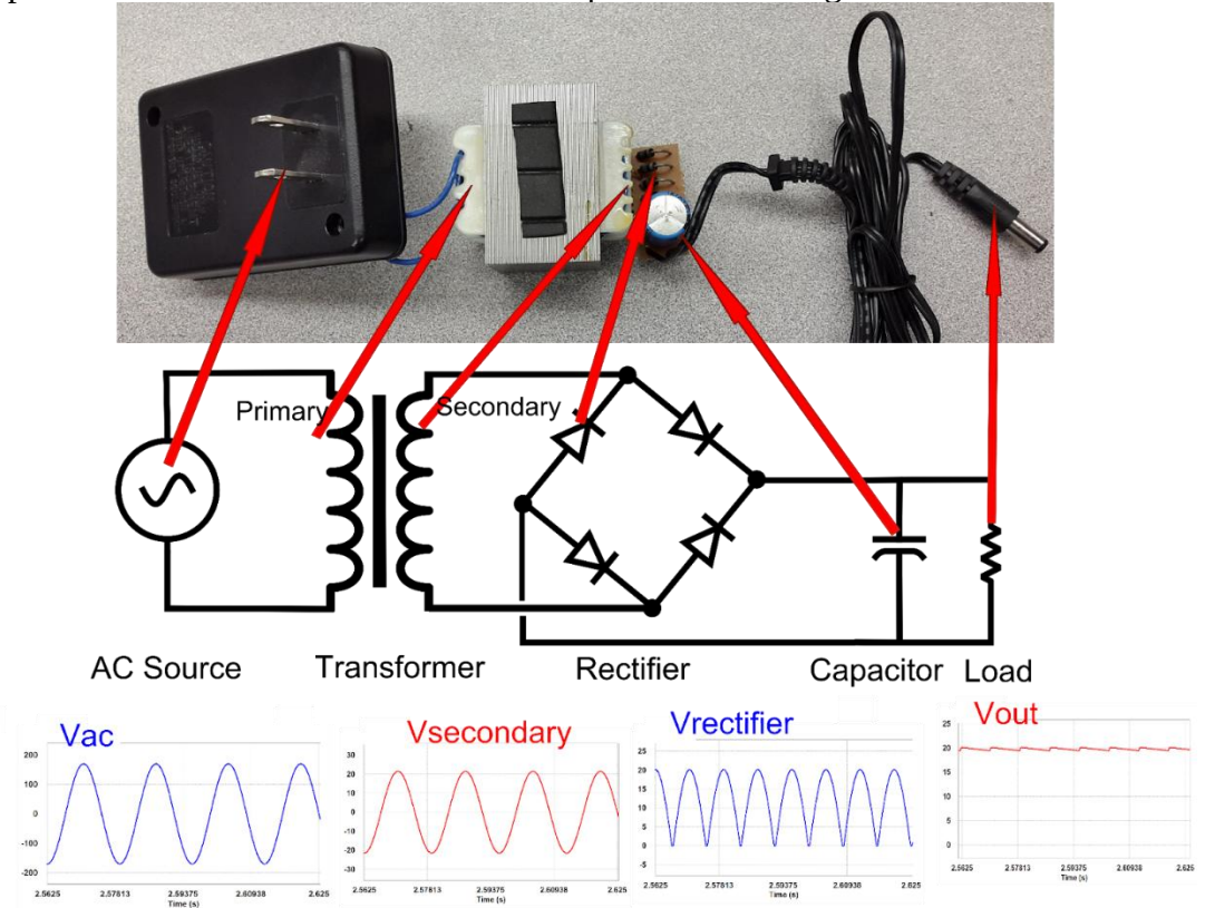
Figure 3-1: Diagram Analysis of AC Power Supply
