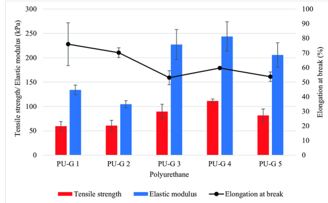
Figure 0-2: Tensile strength of different polyurethanes produced by different water content
