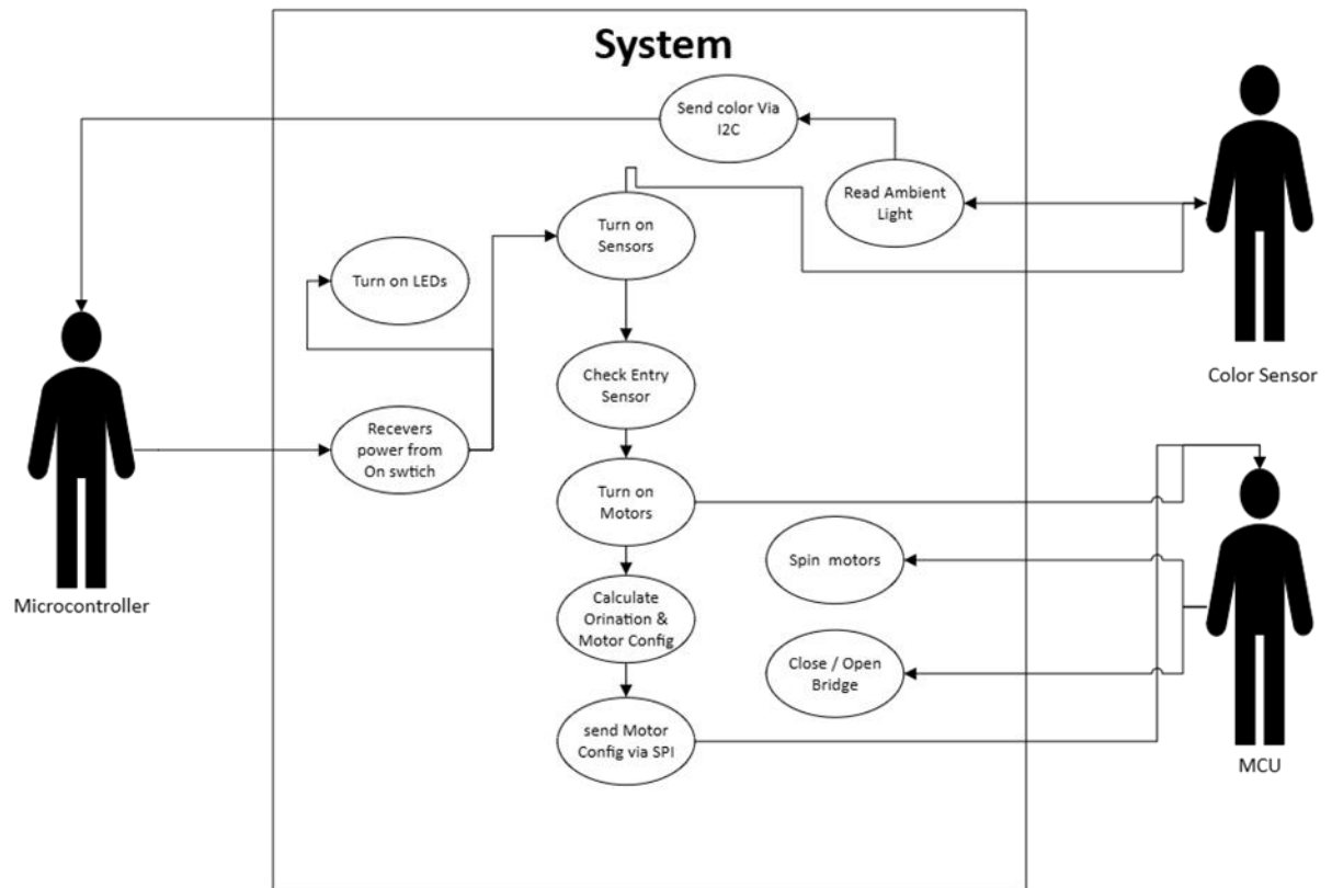
Figure 7-1: User Diagram
